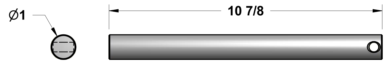
C-15244 CONNECTING PIN
