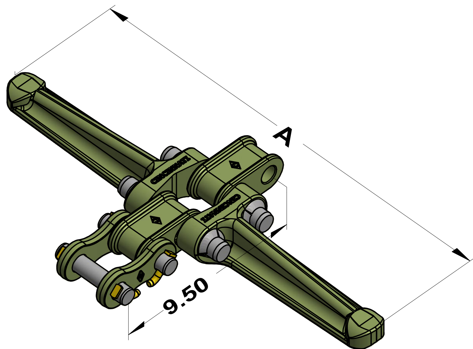
DA-4342 CHAIN UNIT
