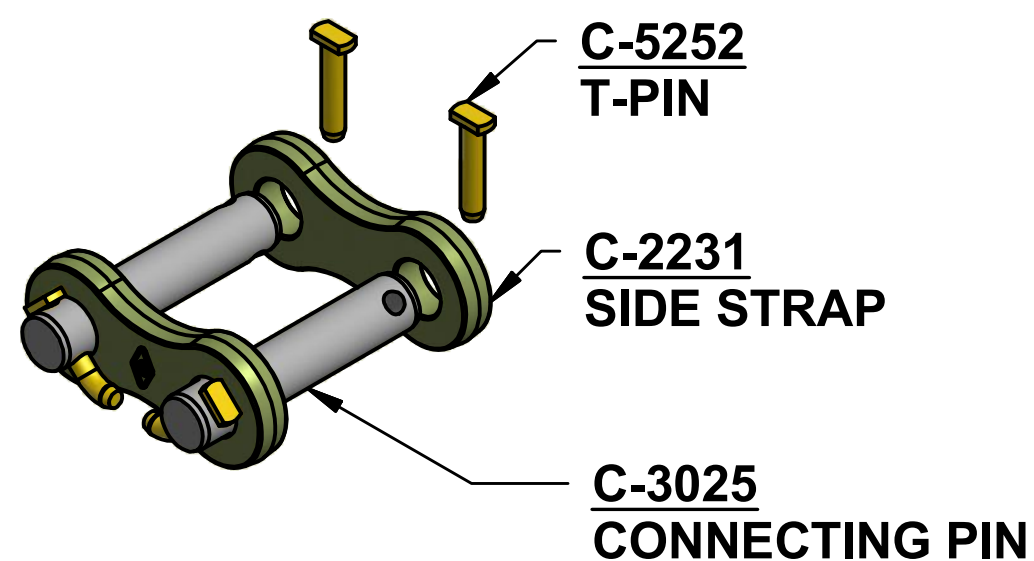
C-11514 DA-434 SIDE STRAP ASSEMBLY (or connecting links)
