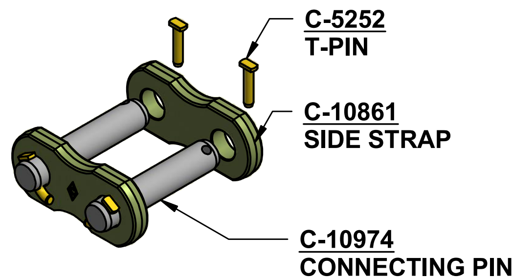
C-11187 DA-615 SIDE STRAP ASSEMBLY (or connecting links)
