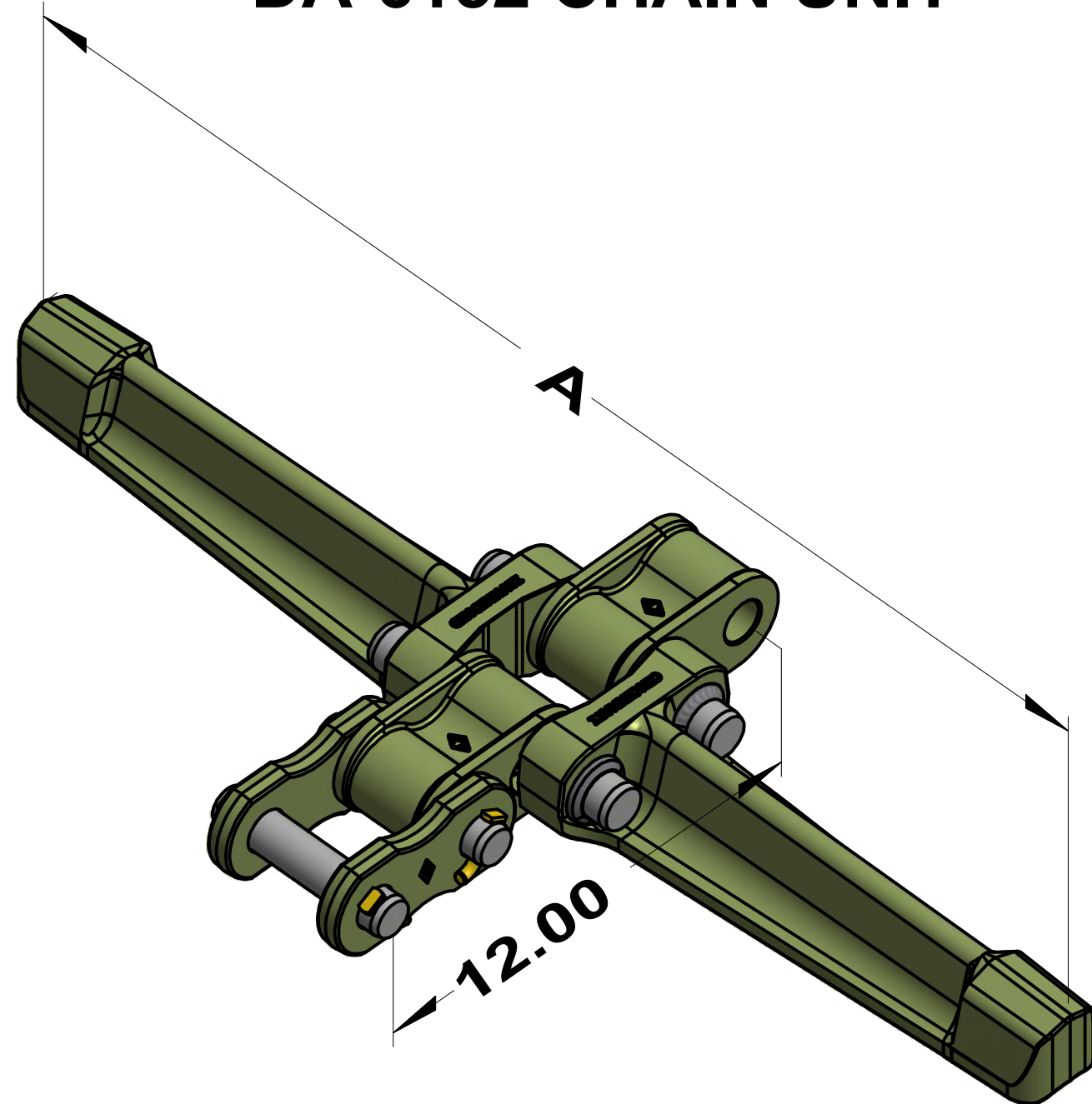
DA-6152 CHAIN UNIT
