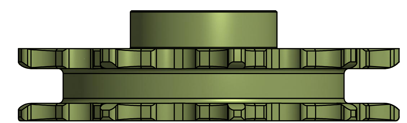
G-1108 9 TOOTH SPROCKET
